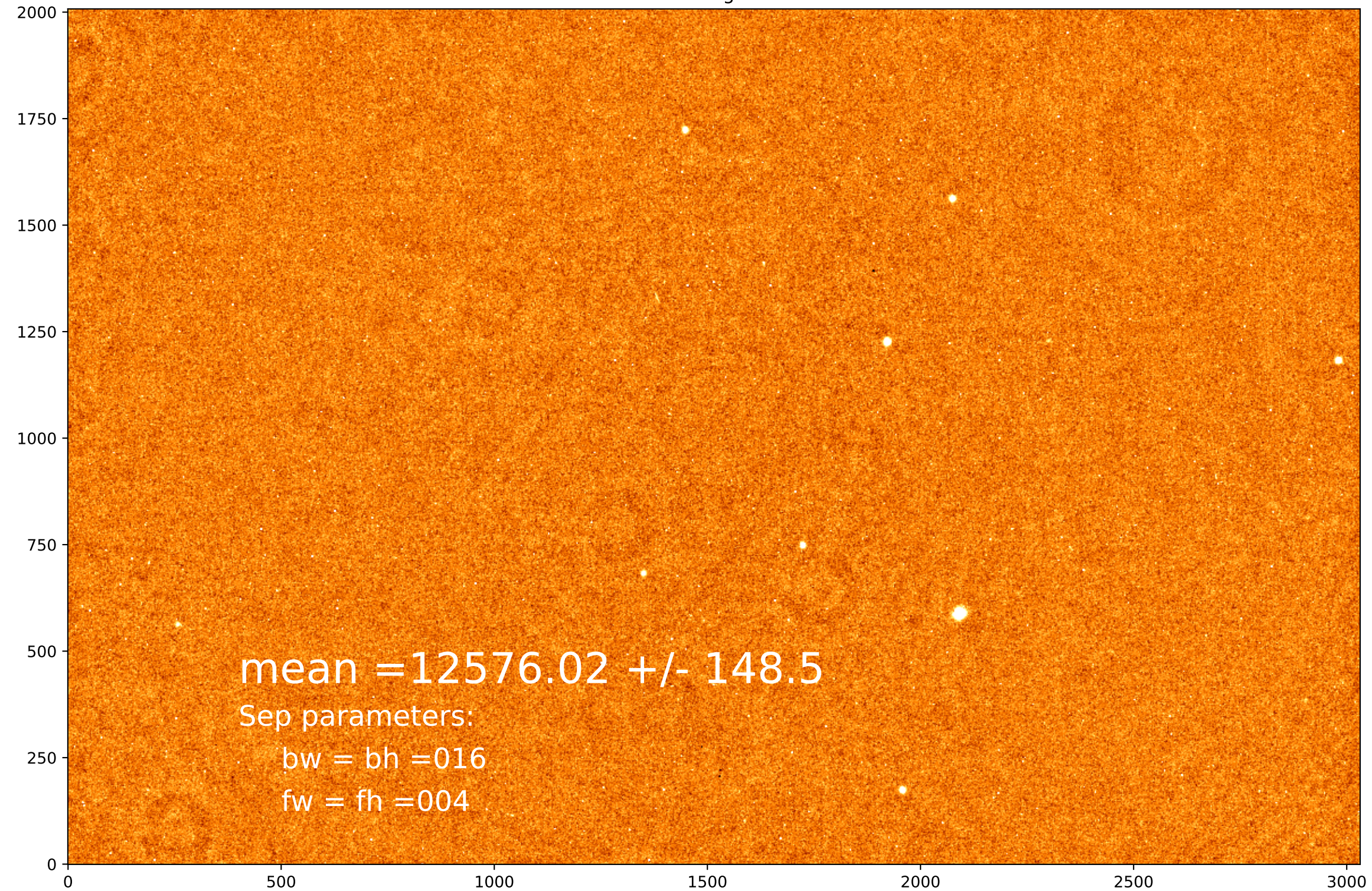
Pseudo-flat-fielded image with linear stretch
