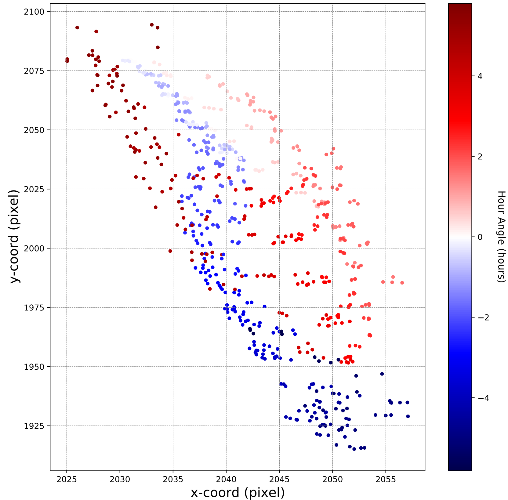
(x,y) coordinates of nominal ( \alpha, \delta )
